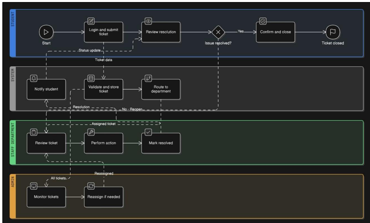
Activity Diagram
