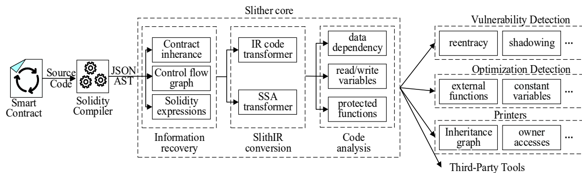
Figure 23. Slither overview.
