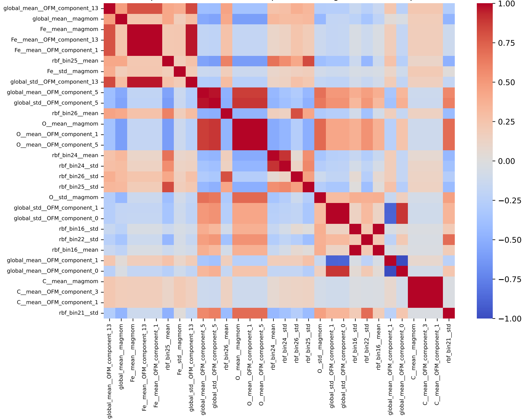
Descriptor correlation matrix (top 30 OFM/magmom/rbf descriptors)
