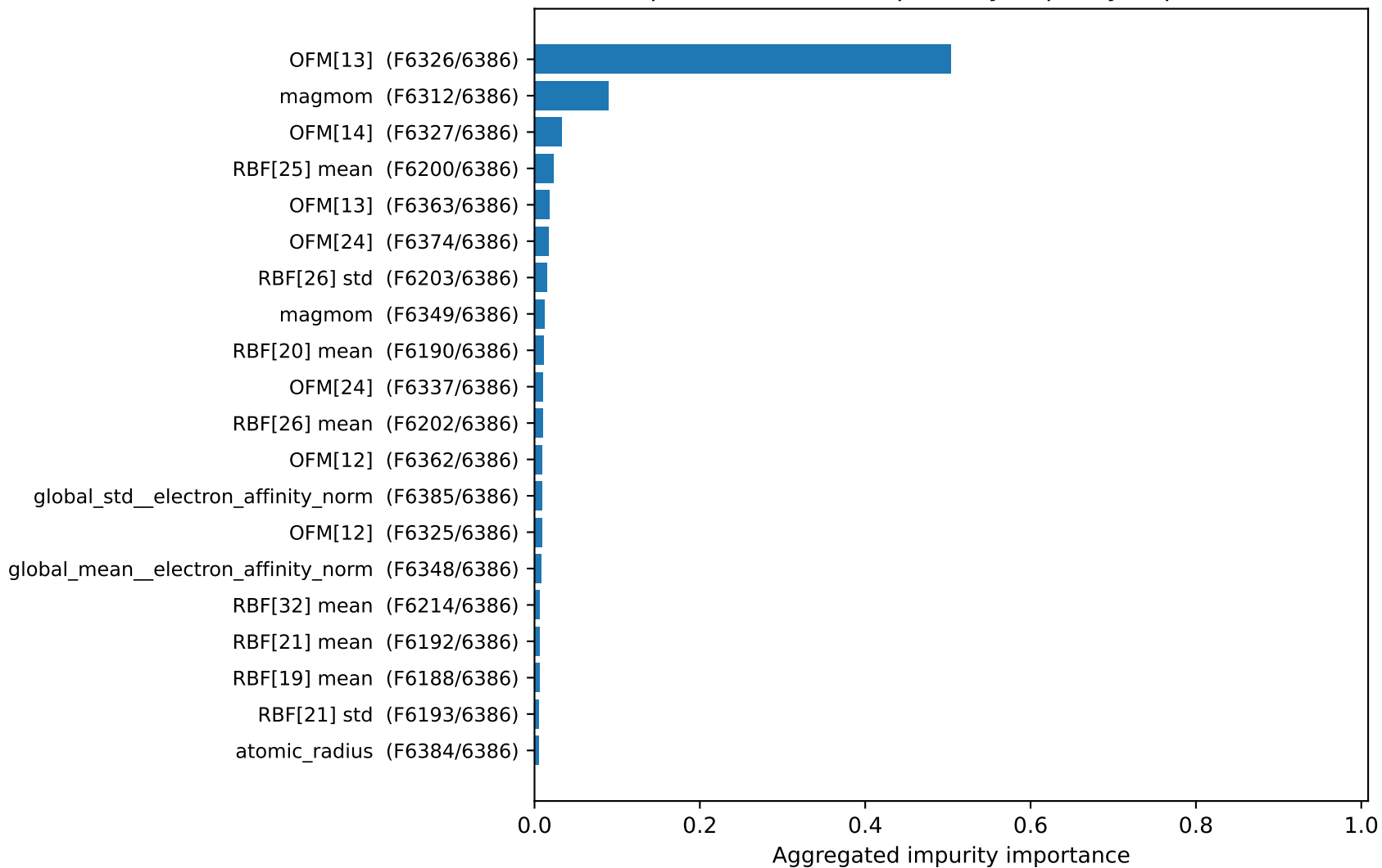
Top-20 CGVEC descriptors by impurity importance
