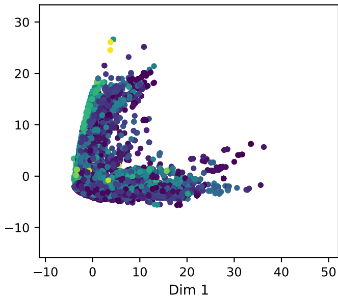
conv_3
