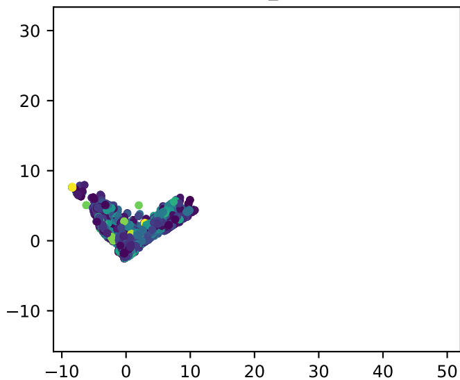
conv_3
