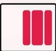
flex-end
