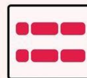
space-around
