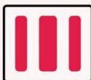
space-evenly
