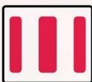
space-between
