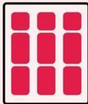
column
