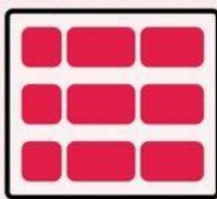
row
