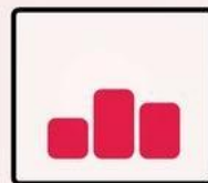
flex-end
