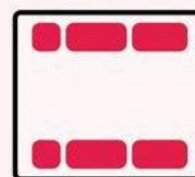
space-between
