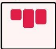
flex-start
