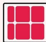
stretch
