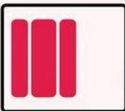
flex-start
