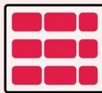
row-reverse
