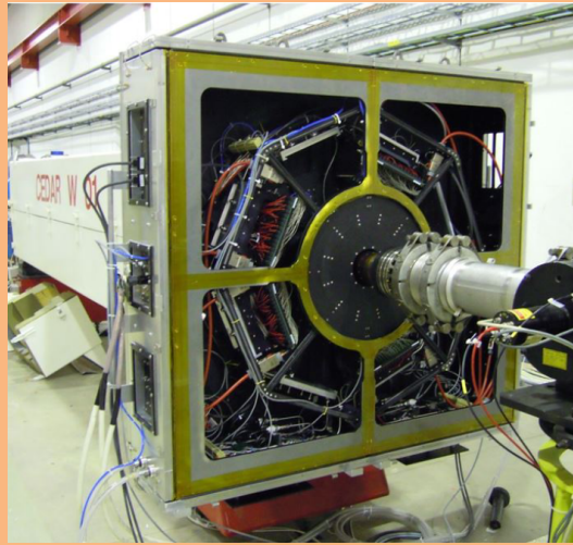
Figure 6: Photo of CEDAR and KTAG installed in the NA62 beamline
