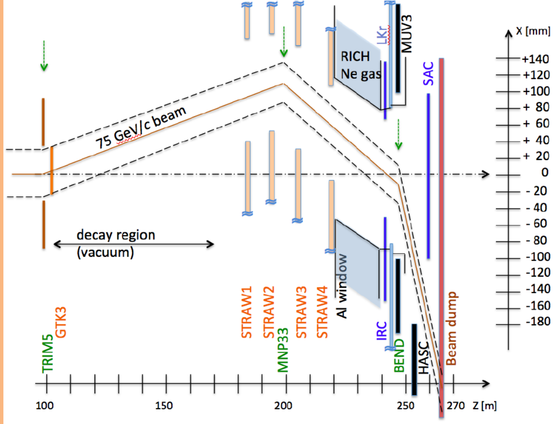
Figure 4: Schematic of K12 beamline after GTK3 (2).
