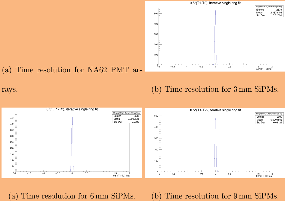
Figure 12: Time resolution for NA62 PMTs and the three possible HIKE SiPMs, calculated from the time difference between two equally populated subset of hits within the ring candidate. A detailed description of the procedure is provided here [5]
