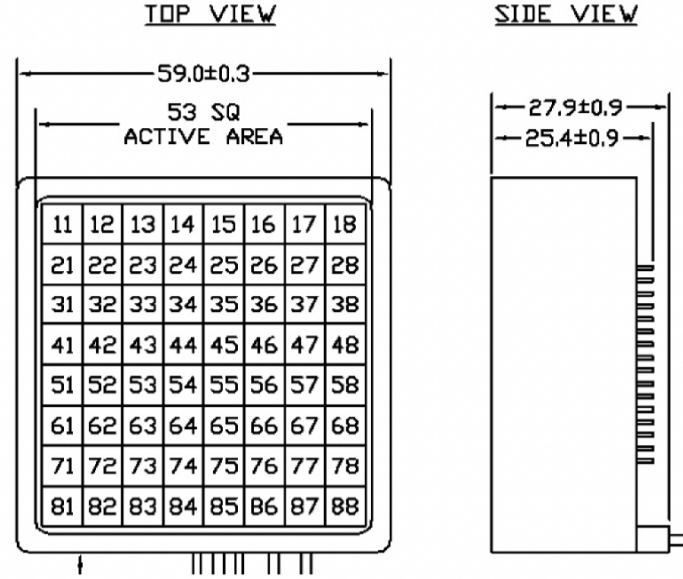
Figure 6: Schematic of Photonics MCP-PMT [5]
