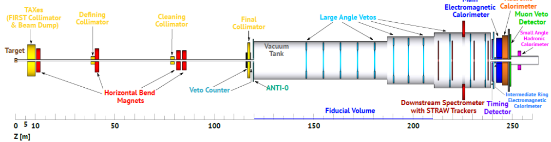
Figure 3: Diagram of HIKE Phase 2 detector setup [1]
