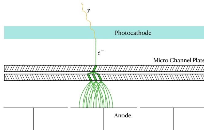
Figure 5: Diagram describing the workings of a MCP-PMT.
