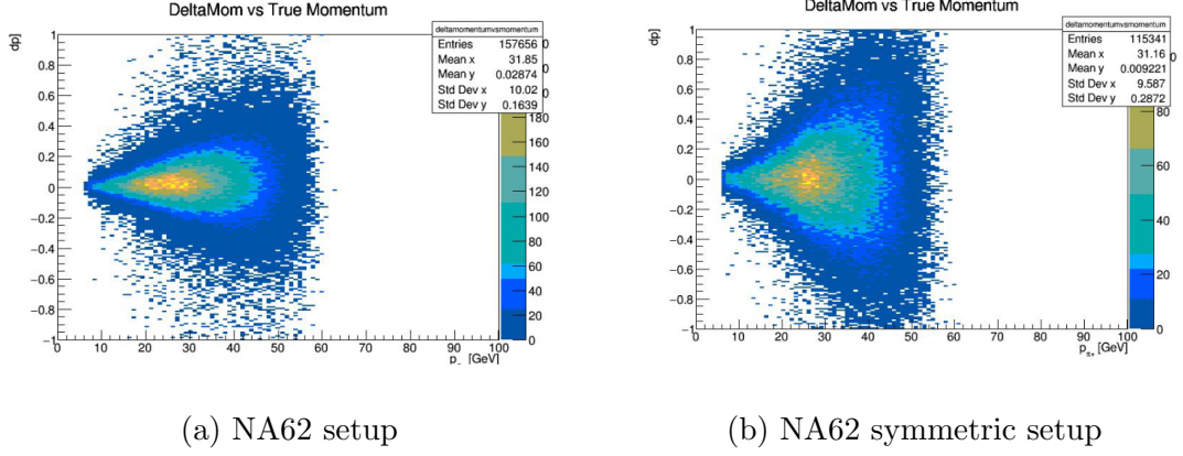
Figure 14: Difference between reconstructed and true pion momentum against true pion momentum from K \rightarrow \pi^+ 0 \text{decay}
