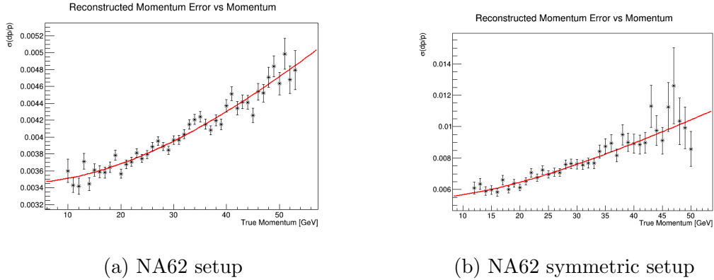
Figure 15: Sigma of fitted Gaussian of the reconstructed and true pion momentum against true pion momentum from K \rightarrow \pi^+ 0 \text{decay}
