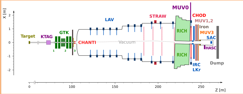
Figure 3.2: X-Z diagram of NA62 detector setup for Run 1
