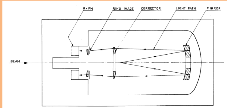
Figure 3.5: Diagram describing the CEDAR optics ?
