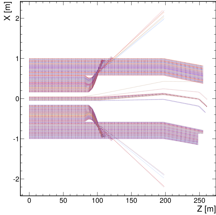
Figure 5: Traks for charged Geantinos with a 400 GeV/c momentum through the NA62 detector.
