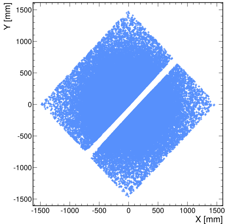
Figure 2: Geantino hits on a single view in STRAW chamber 1.
