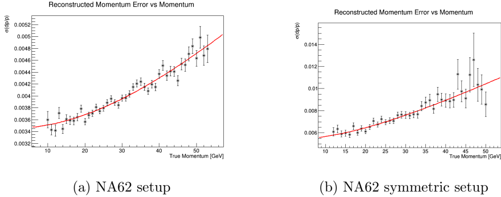
Figure 15: Sigma of fitted Gaussian of the reconstructed and true pion momentum against true pion momentum from K \rightarrow \pi^+\pi^0 decay
