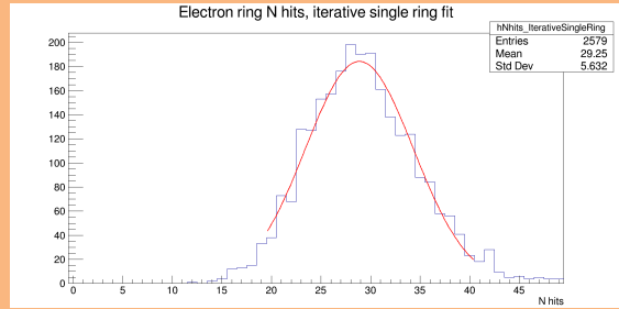
(a) Number of hits per ring candidate for NA62 PMT arrays. (b) Number of hits per ring candidate for 3 mm SiPMs, = 28.86.
