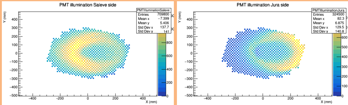
(a) Light distribution for NA62 setup on the Saleve side of the RICH detector. (b) Light distribution for NA62 setup on the Jura side of the RICH detector.
