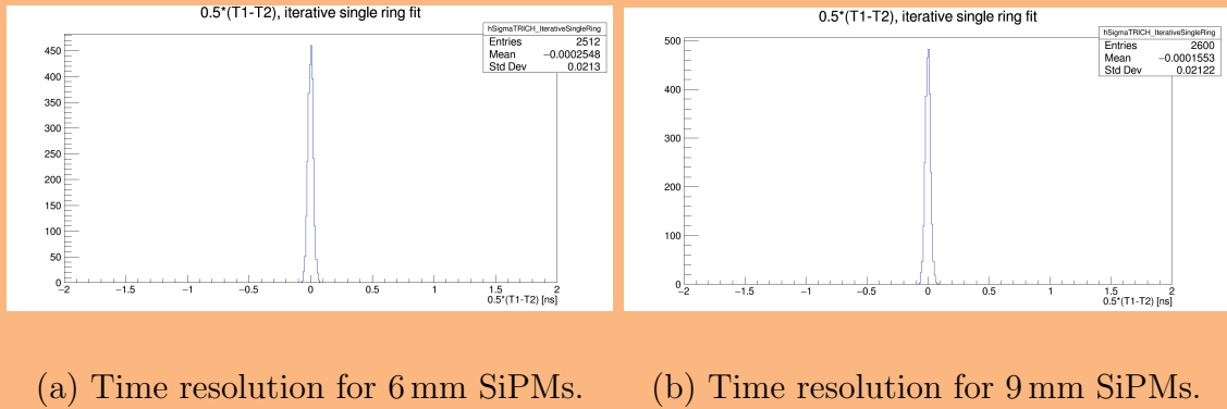
Figure 13: Time resolution for NA62 PMTs and the three possible HIKE SiPMs, calculated from the time difference between two equally populated subset of hits within the ring candidate. A detailed description of the procedure is provided here [5]
