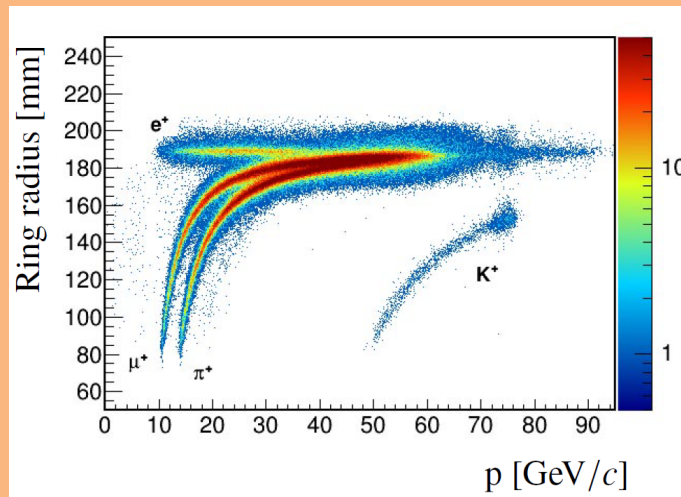
Figure 3.12: Cherenkov ring radius as a function of the particle momentum ?
