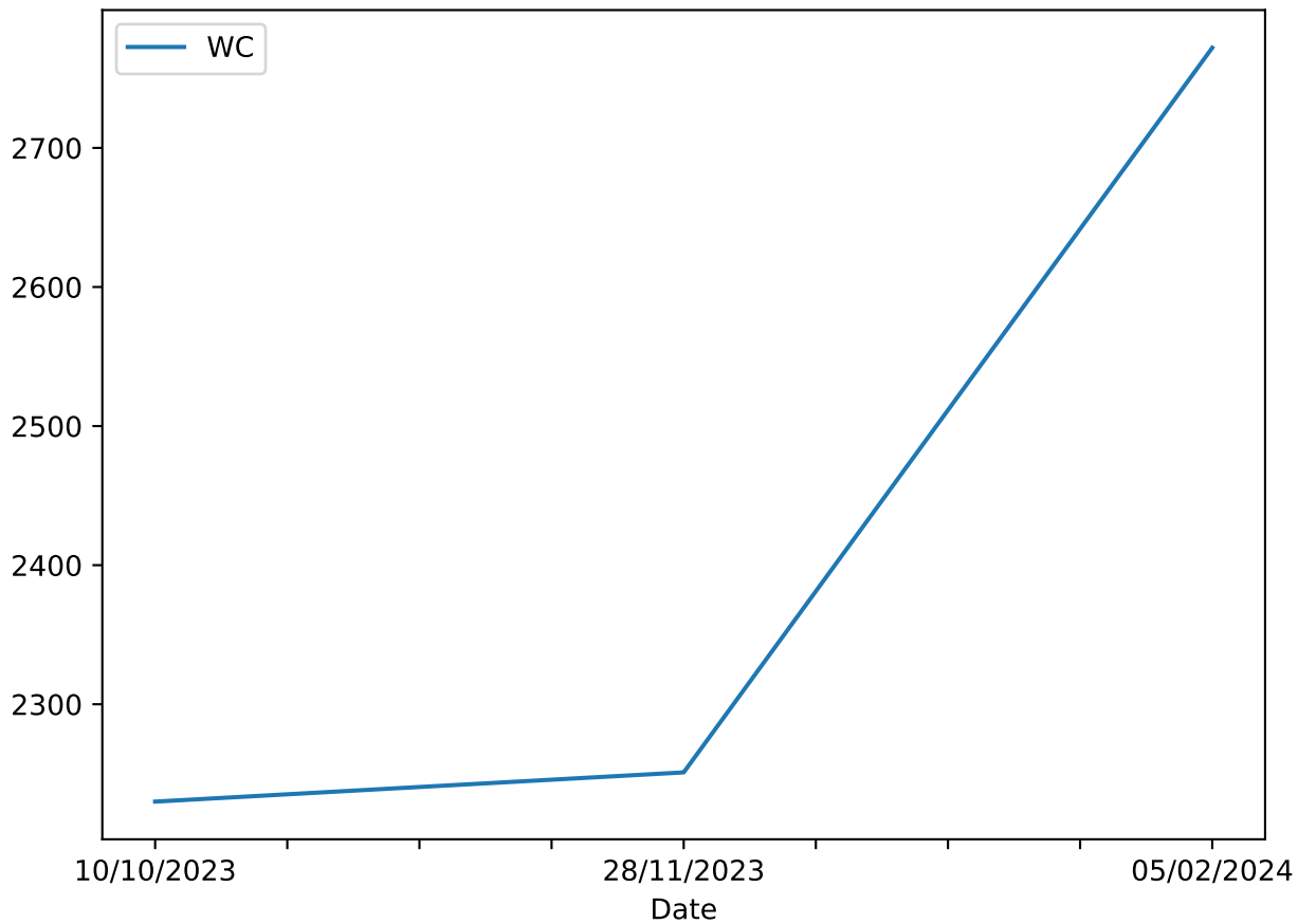
Word Count vs Date
