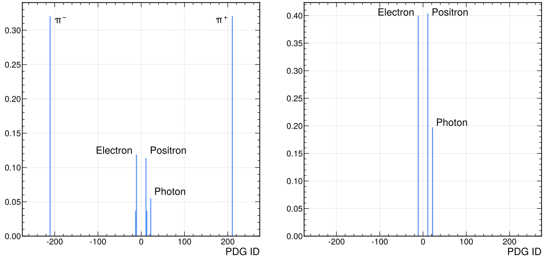
Figure 20: Monte Carlo particle code for the particles producing a hit in the Spectrometer. Left, for the K_L \rightarrow \pi^+ \pi^- \pi^0 decay and right, for the K_L \rightarrow \pi^0 \pi^0 \pi^0 decay.
