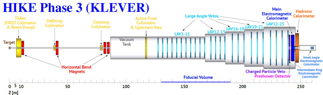
Figure 4: Diagram of HIKE phase 3 detector setup [1]
