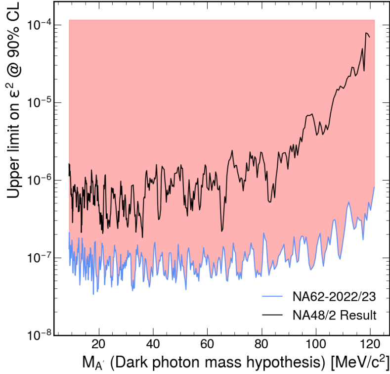
Figure 25: Upper limit mixing parameter \epsilon^2 at a 90% CL for each Dark Photon mass value from the data driven background estimation, with the result from NA48/2 for comparison [1].
