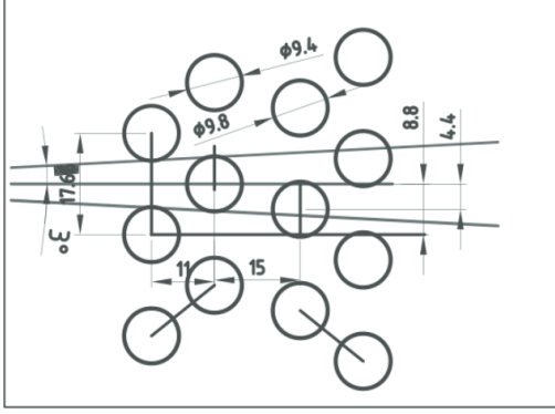
Figure 9: Diagram of straw placement in each view [5]
