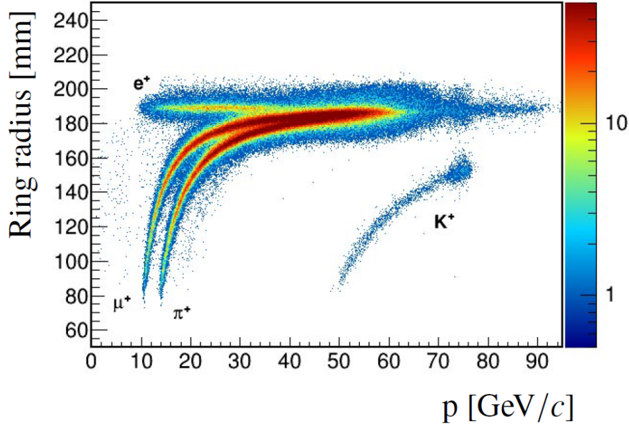
Figure 12: Cherenkov ring radius as a function of the particle momentum [6]
