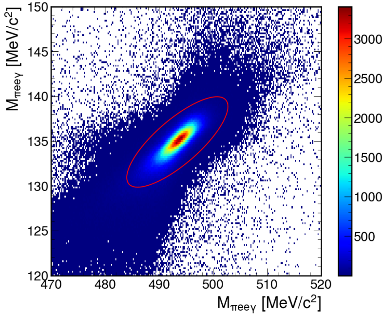
Figure 3: Reconstructed missing mass of M_{\pi ee\gamma} compared against M_{ee\gamma} produced from a K2pi Dalitz MC sample, with the defined elliptical cut used in the selection
