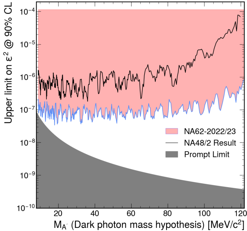
Figure 27: Upper limit mixing parameter \epsilon^2 at a 90% CL for each Dark Photon mass value from the data driven background estimation, with the result from NA48/2 for comparison [?] and the expected limit of the prompt decay.
