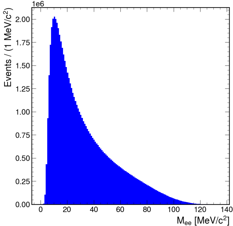
Figure 19: Reconstructed invariant mass of electron-positron pair for events passing the selection from the 2022 and 2023 NA62 dataset.
