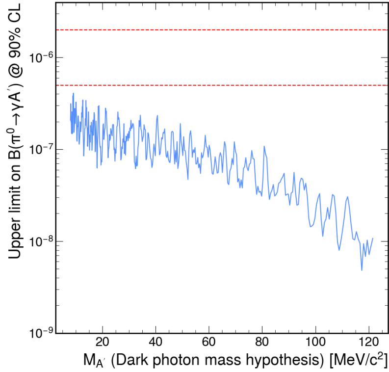
Figure 24: Upper limit on the branching fraction of \pi^0 \rightarrow \gamma A' at a 90% CL for each Dark Photon mass value, for the data driven background method for estimating the number of expected events.
