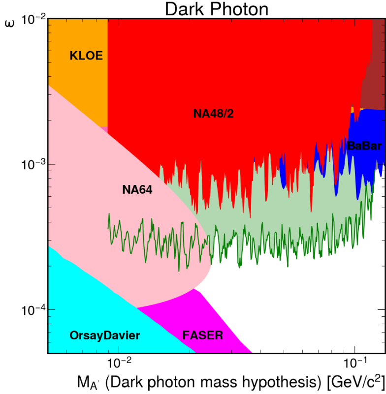
Figure 26: Upper limit at a 90% CL on the mixing parameter for the data driven background estimate (Green) compared to published exclusions limits [? ? ? ? ? ? ? ? ? ]
