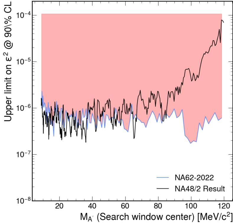
Figure 18: Upper limit mixing parameter \epsilon^2 at a 90% CL for each Dark Photon mass value with the result from NA48/2 for comparison [? ].
