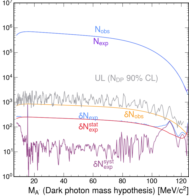
Figure 22: Number of observed data events ( N_{obs} ), expected number of events from the data driven method ( N_{exp} ), the respective errors ( \delta N_{obs} and \delta N_{exp} ) and the resultant upper limit on the number of Dark Photon candidates to a 90% confidence level.
