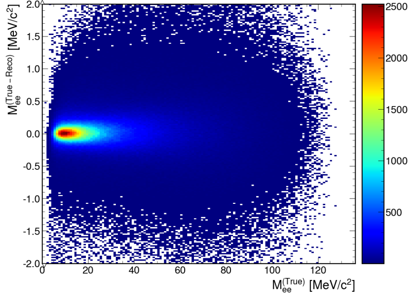
Figure 13: True invariant mass minus reconstructed invariant mass of the electron positron pair in terms of true invariant mass.
