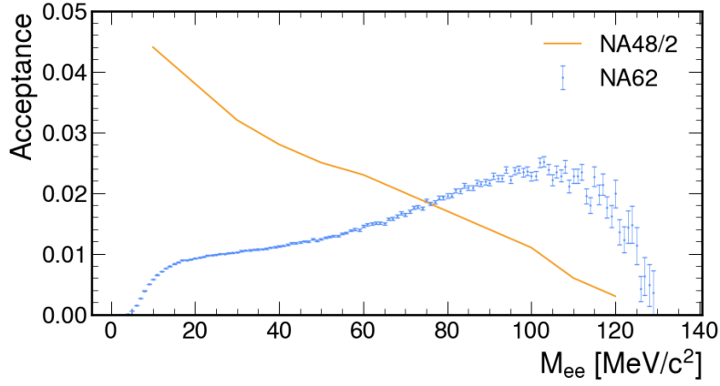
Figure 4: Acceptance of the NA62 selection compared against the acceptance produced in the NA48/2 analysis [? ]
