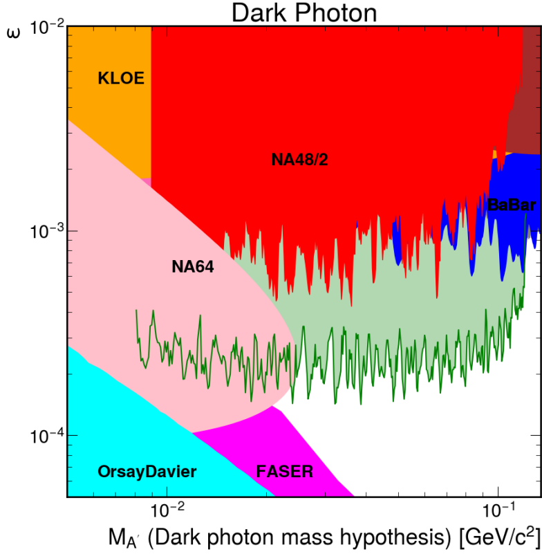
Figure 26: Upper limit at a 90% CL on the mixing parameter for the data driven background estimate (Green) compared to published exclusions limits [1, 10, 11, 12, 13, 14, 15, 16]
