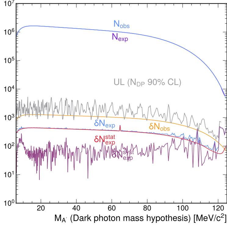
Figure 22: Number of observed data events ( N_{\text{obs}} ), expected number of events from the data driven method ( N_{\text{exp}} ), the respective errors ( \delta N_{\text{obs}} and \delta N_{\text{exp}} ) and the resultant upper limit on the number of Dark Photon candidates to a 90% confidence level.
