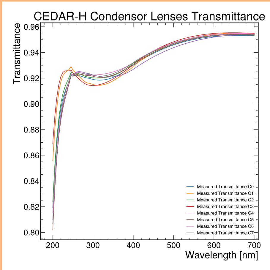
Figure 4.2: Measured transmittance of CEDAR-H condensor lenses conducted by Thomas Schneider at CERN
