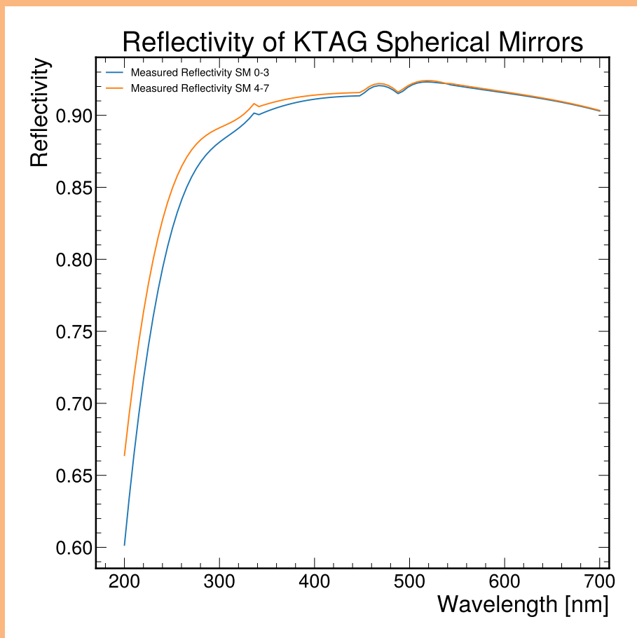
Figure 4.4: Measured reflectivity of KTAG spherical mirror conducted by Thomas Schneider at CERN
