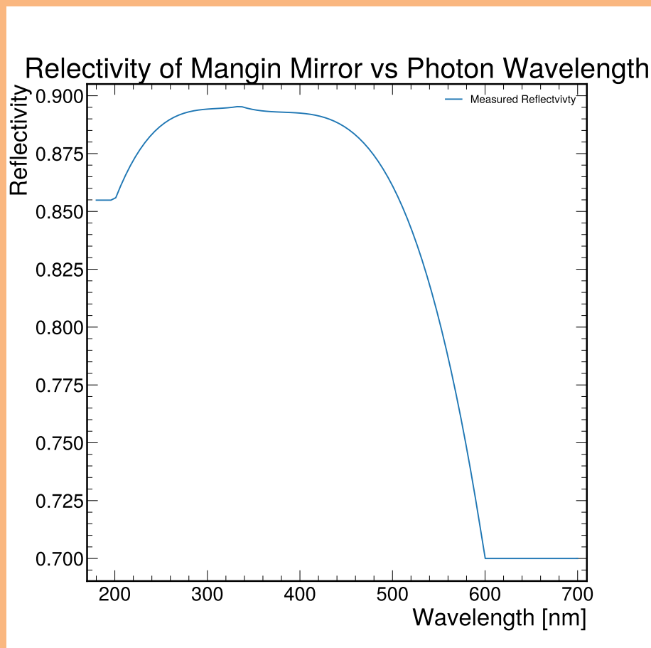
Figure 4.1: Measured reflectivity of CEDAR-H mangin mirror conducted by Win-light System
