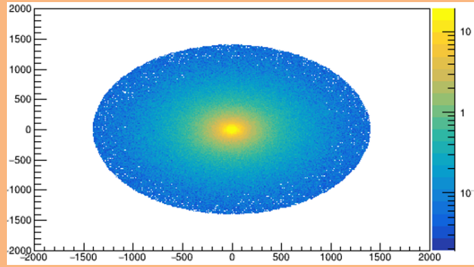
Figure 16: Rate of particles across the cross section at the first STRAW chamber entrance at Z=213.\text{m} .
