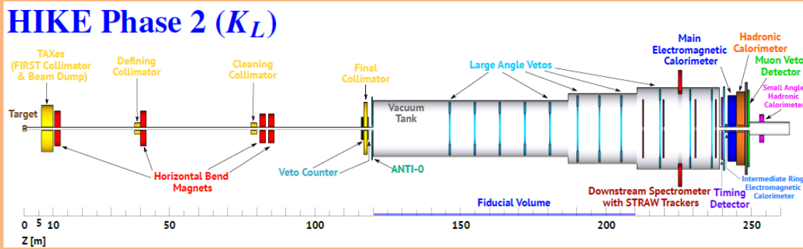
Figure 3: Diagram of HIKE phase 2 detector setup [1]
