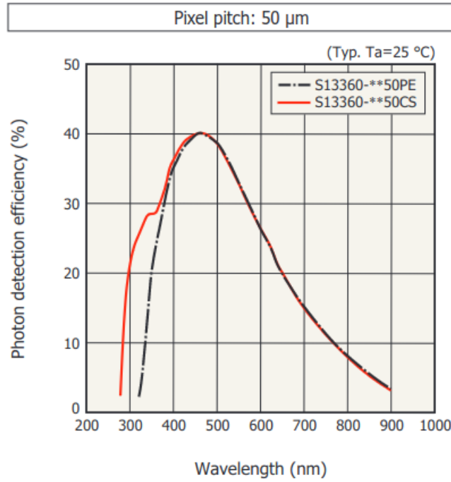
Figure 14: Selected SiPM quantum efficiency taken from Hamamatsu S13360 datasheet [7]
