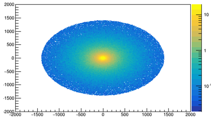
Figure 21: Rate of particles across the cross section at the first STRAW chamber entrance at Z=213 .m.
