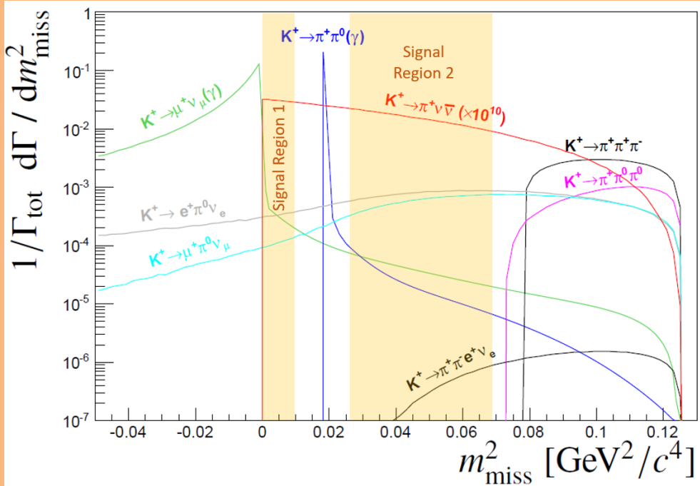
Figure 1: Expected squared missing mass distributions of main kaon decays and K^+ \rightarrow \pi^+ \nu \bar{\nu} (scaled by 10^{10} for for visability). The solid coloured areas show the signal regions used to kinematically reject the domiant kaon decays.
