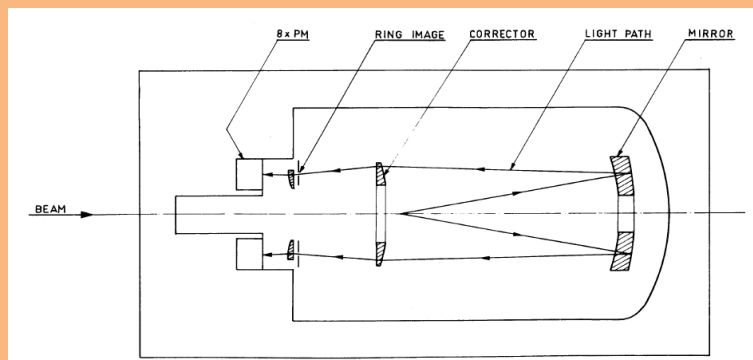
Figure 3.5: Diagram describing the CEDAR optics (1)
