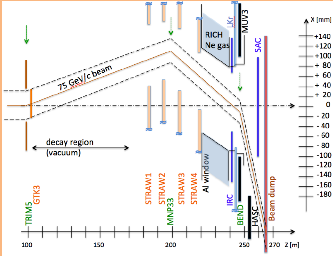
Figure 3.4: Schematic of K12 beamline after GTK3 (3).
