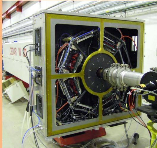
Figure 3.6: Photo of CEDAR and KTAG installed in the NA62 beamline
