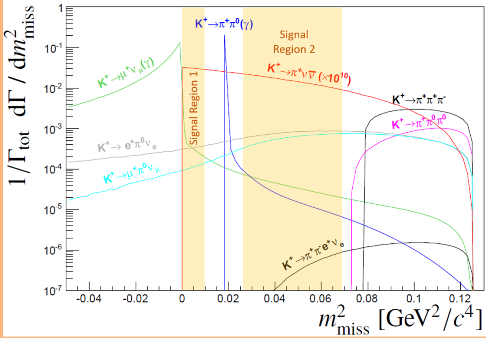
Figure 3.1: Expected squared missing mass distributions of main kaon decays and K^+ \rightarrow \pi^+ \nu \bar{\nu} (scaled by 10^{10} for visibility). The solid coloured areas show the signal regions used to kinematically reject the dominant kaon decays.
