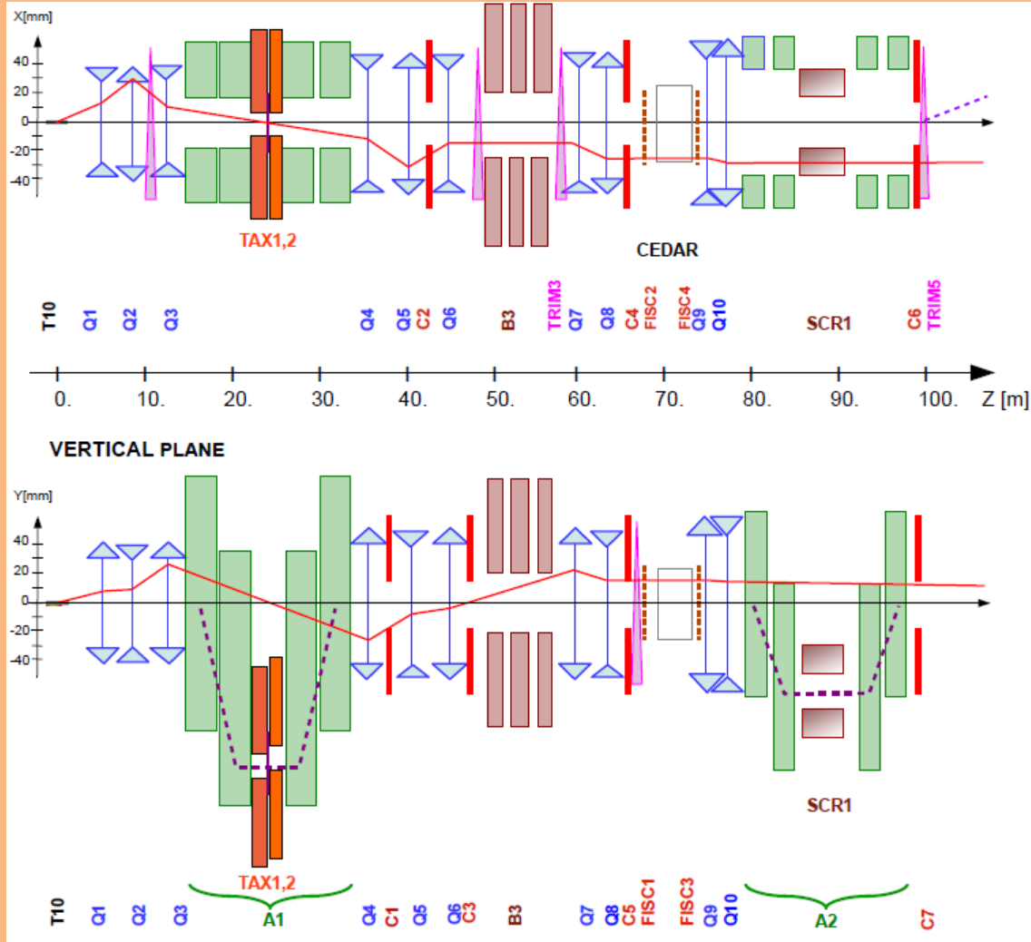
Figure 3.3: Schematic of K12 beamline from T10 target at 0m to the entrance of the NA62 decay region at 102.4m(3).
