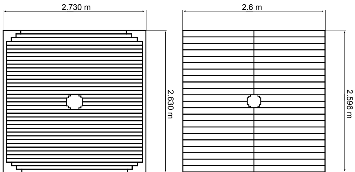
Figure 18: Layout of scintillating tiles for a horizontal layer for: Left, MUV1 and Right, MUV2.
