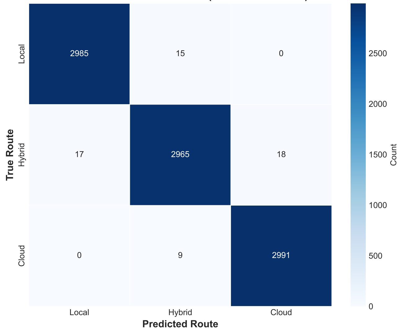
Confusion Matrix — Counts (9K Held-Out Test)
