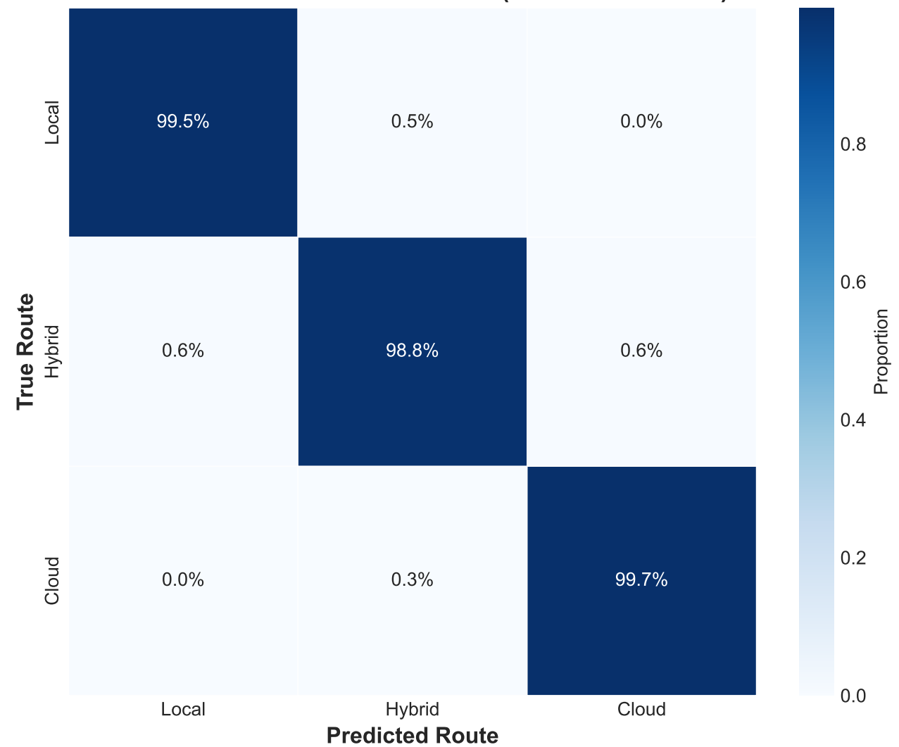
Confusion Matrix — Normalized (9K Held-Out Test)
