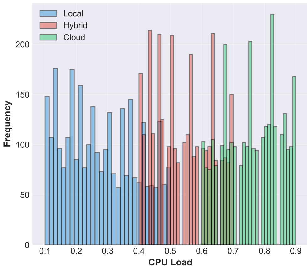
CPU Load Distribution by Route
