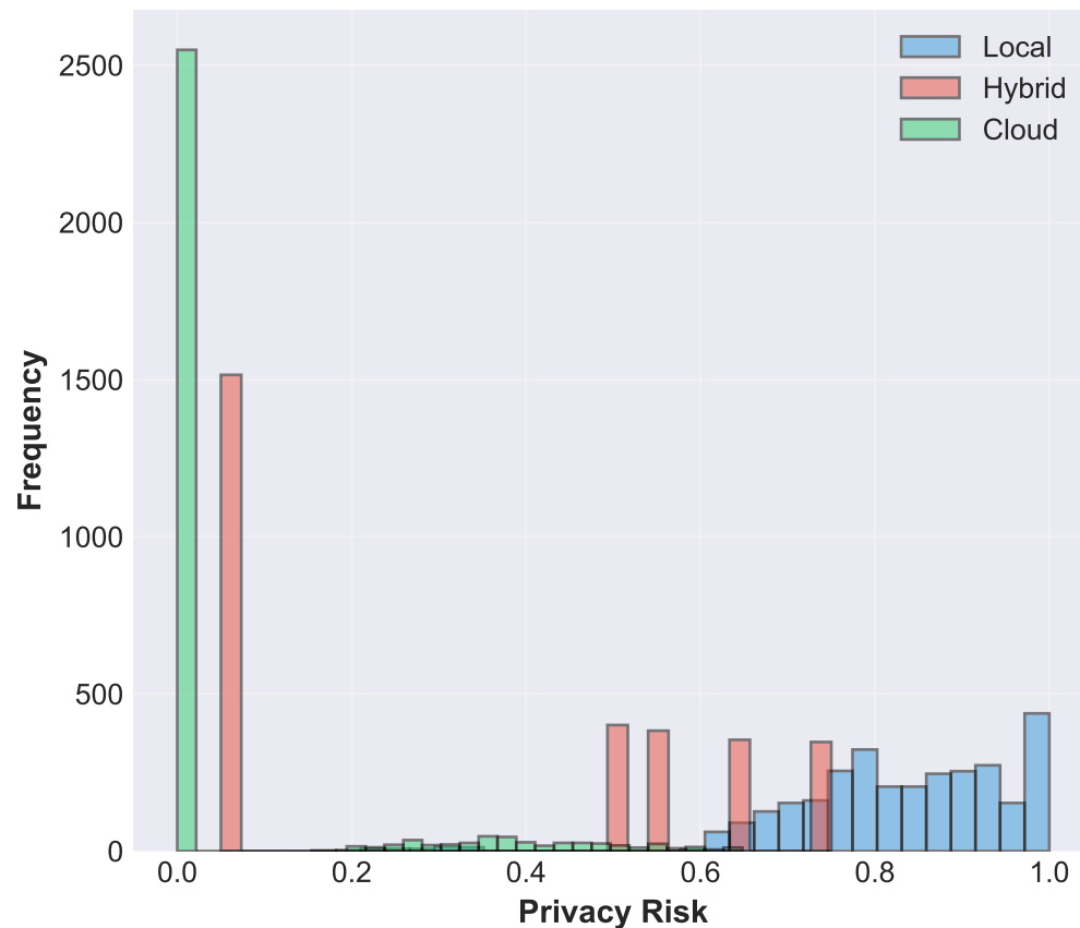
Privacy Risk Distribution by Route
