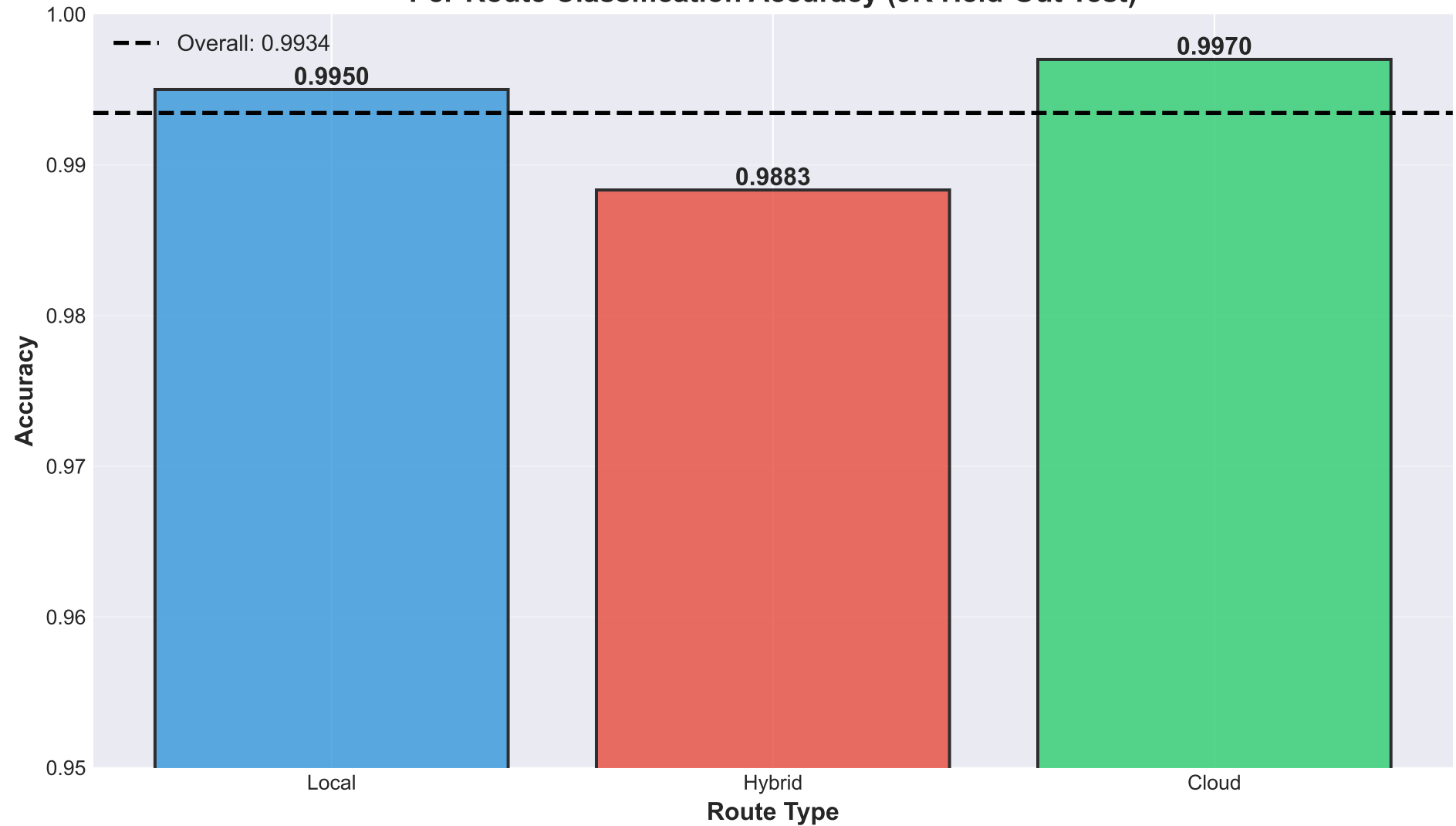
Per-Route Classification Accuracy (9K Held-Out Test)
