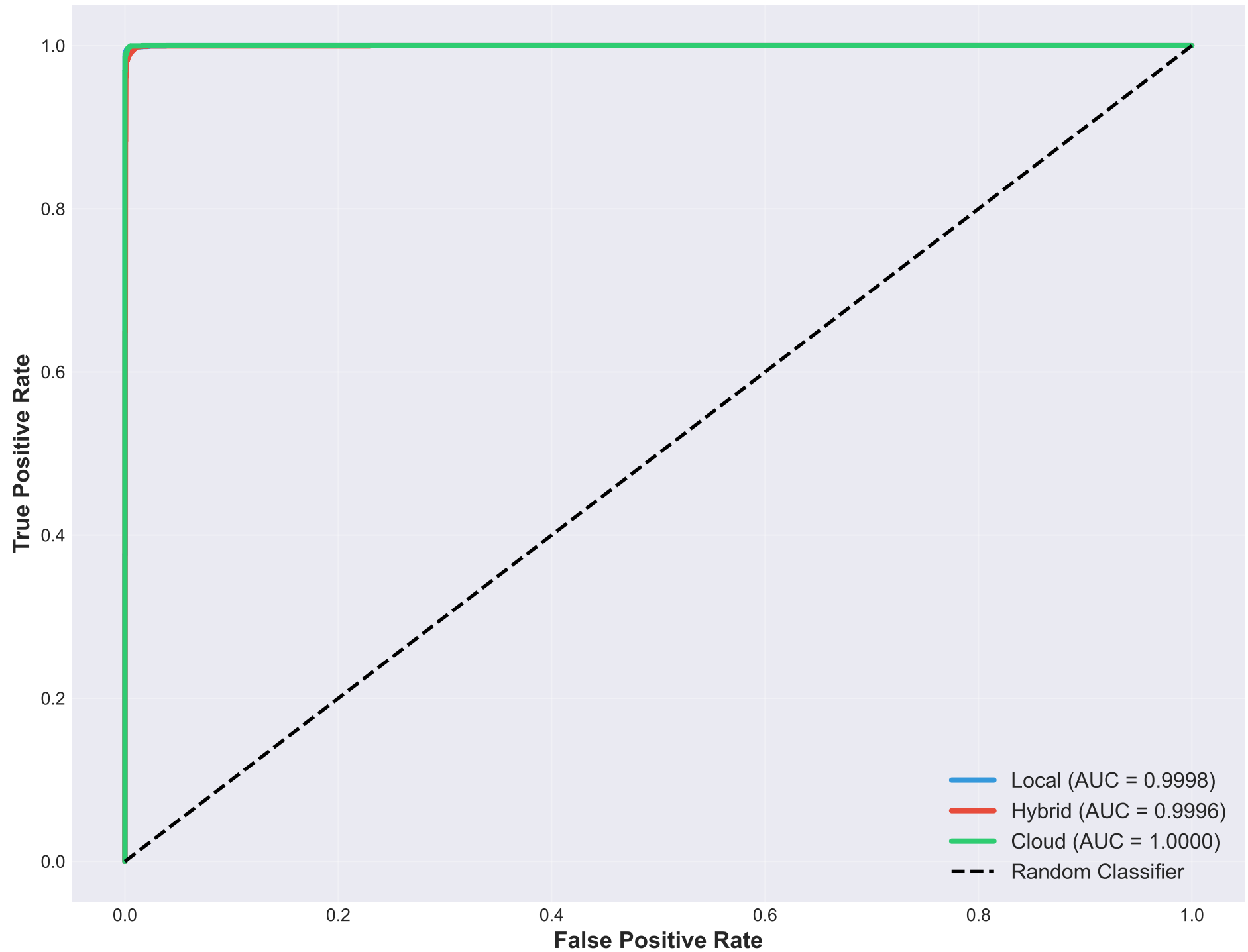
ROC Curves for Multi-class Route Classification (9K Held-Out Test)
