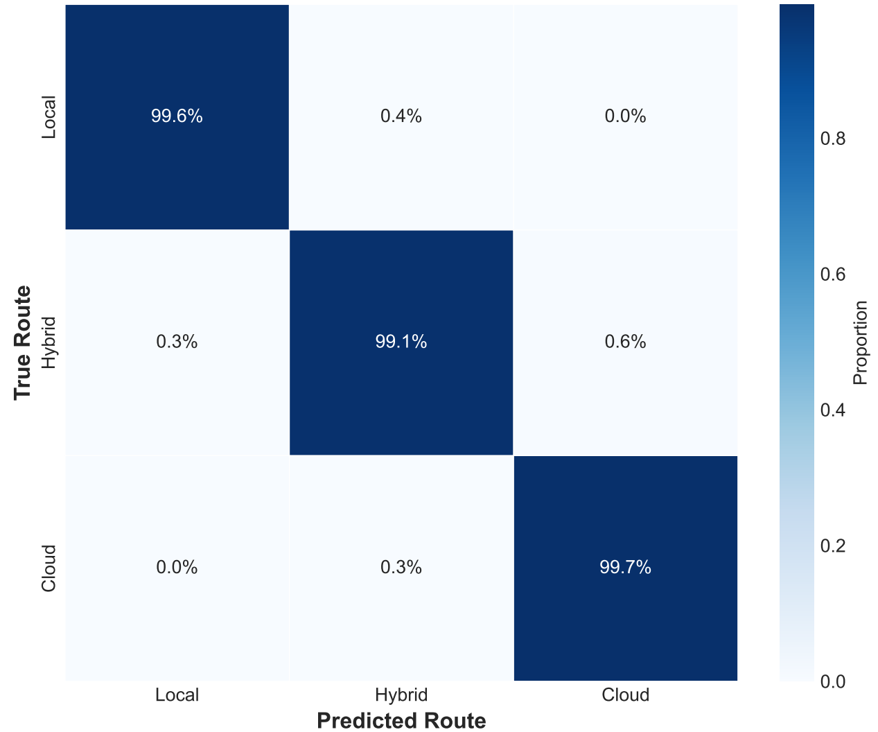
Confusion Matrix — Normalized (75K Training Samples)
