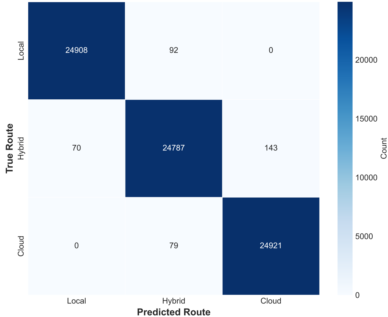
Confusion Matrix — Counts (75K Training Samples)
