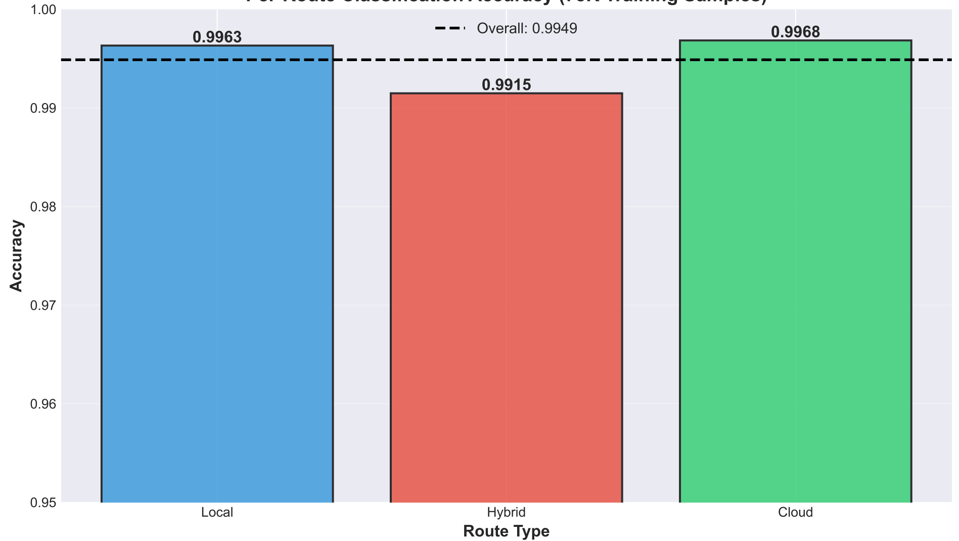
Per-Route Classification Accuracy (75K Training Samples)
