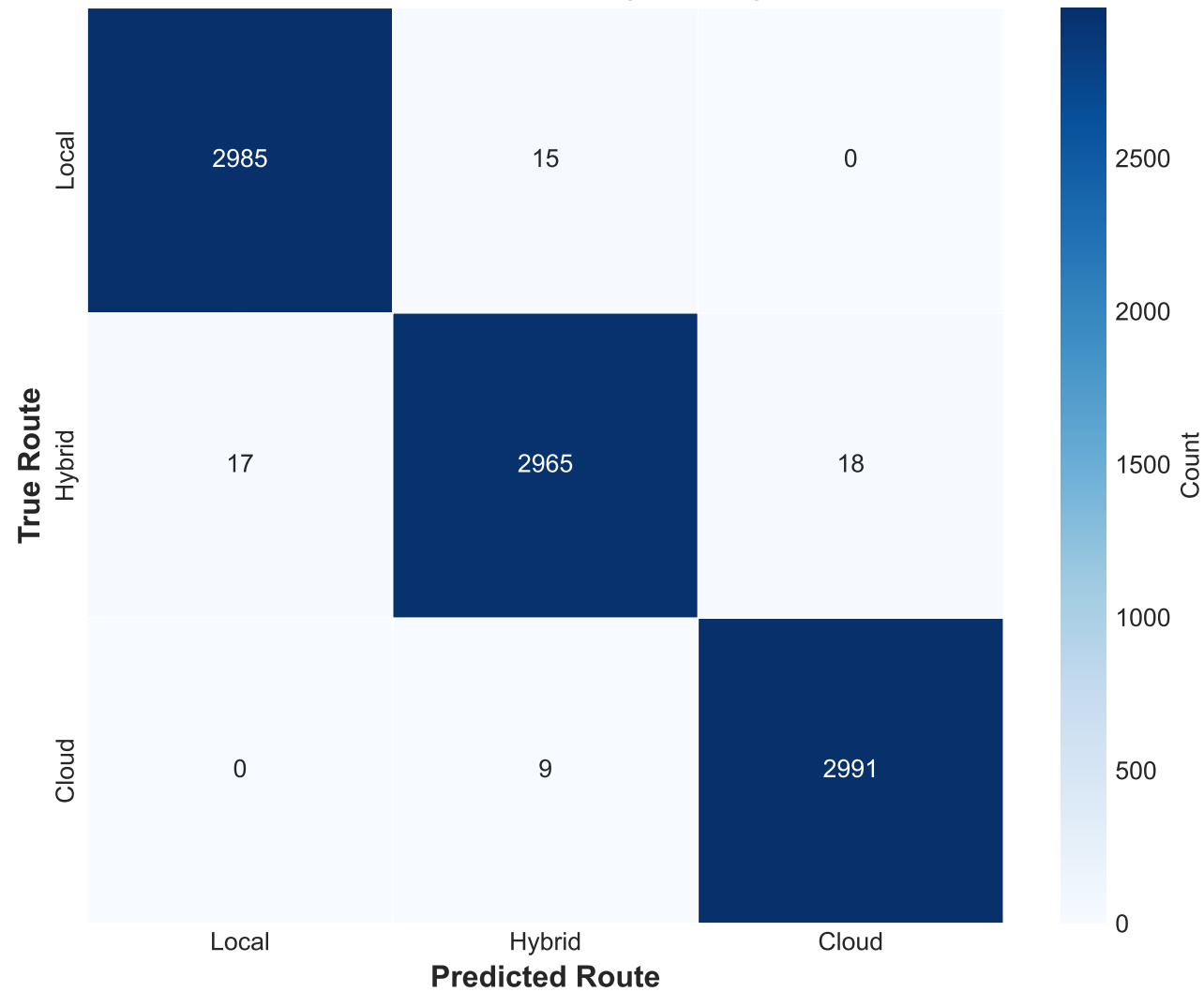
Confusion Matrix (Counts)
