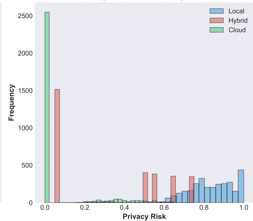
Privacy Risk Distribution by Route
