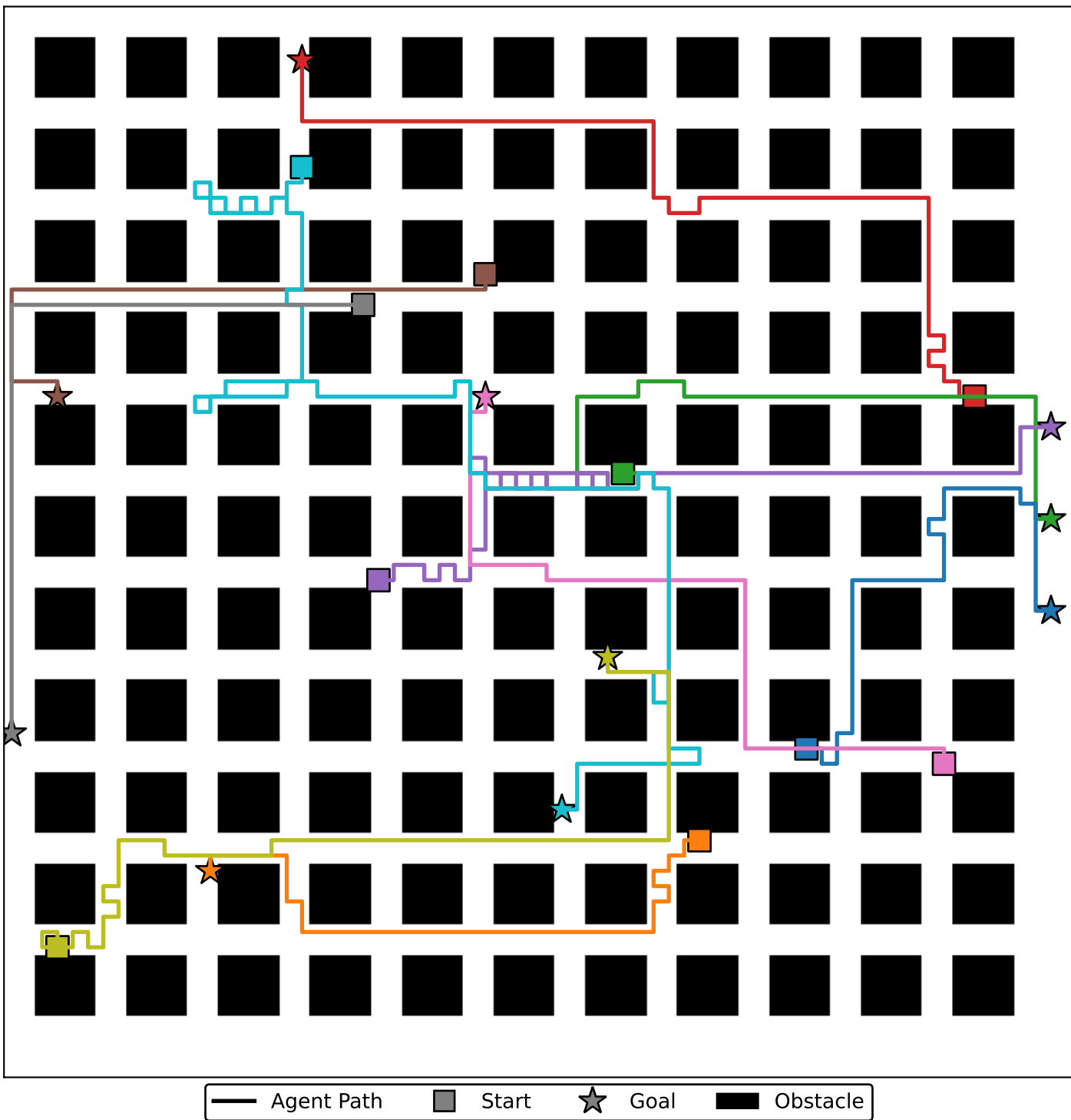
Fixed Structured Grid World 3
