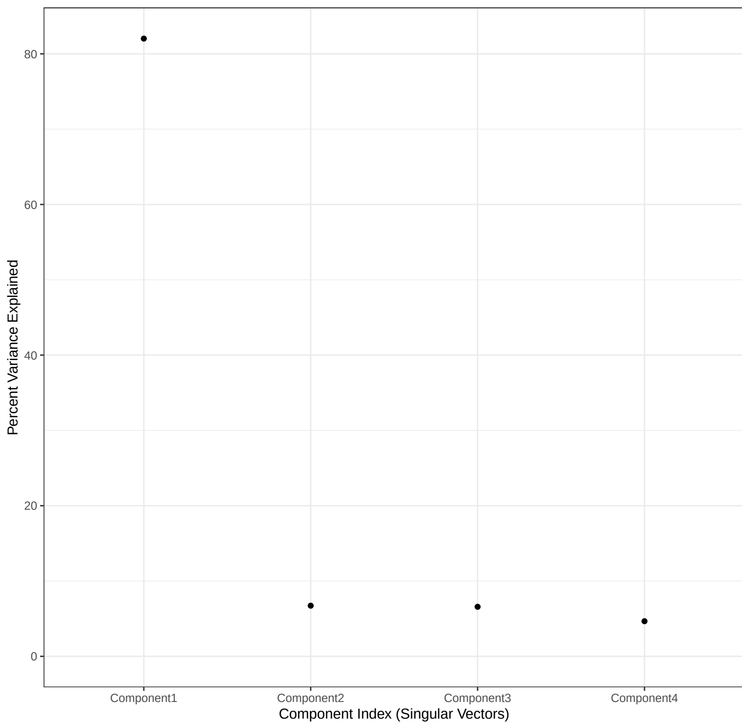
Scree Plot
