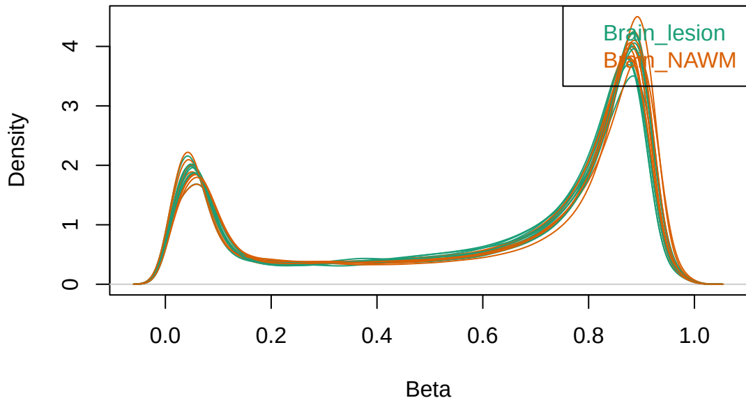
Density plot of raw data (699018 probes)
