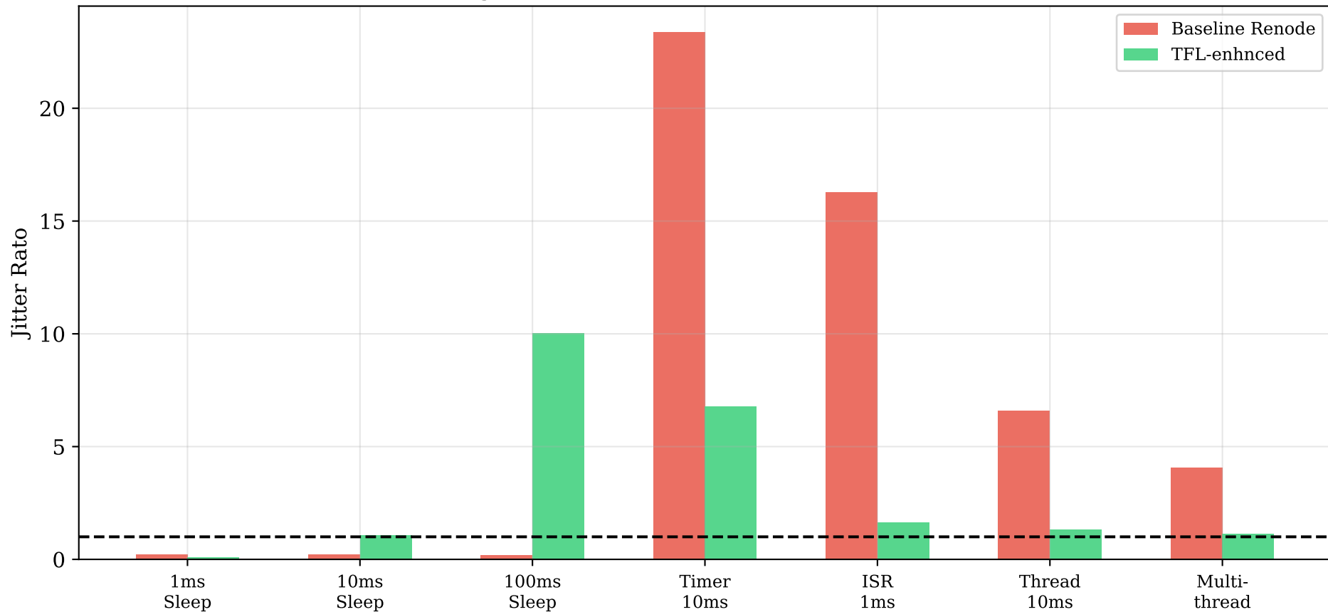
Figure 6.3: Jitter Ratio - Baseline vs TFL
