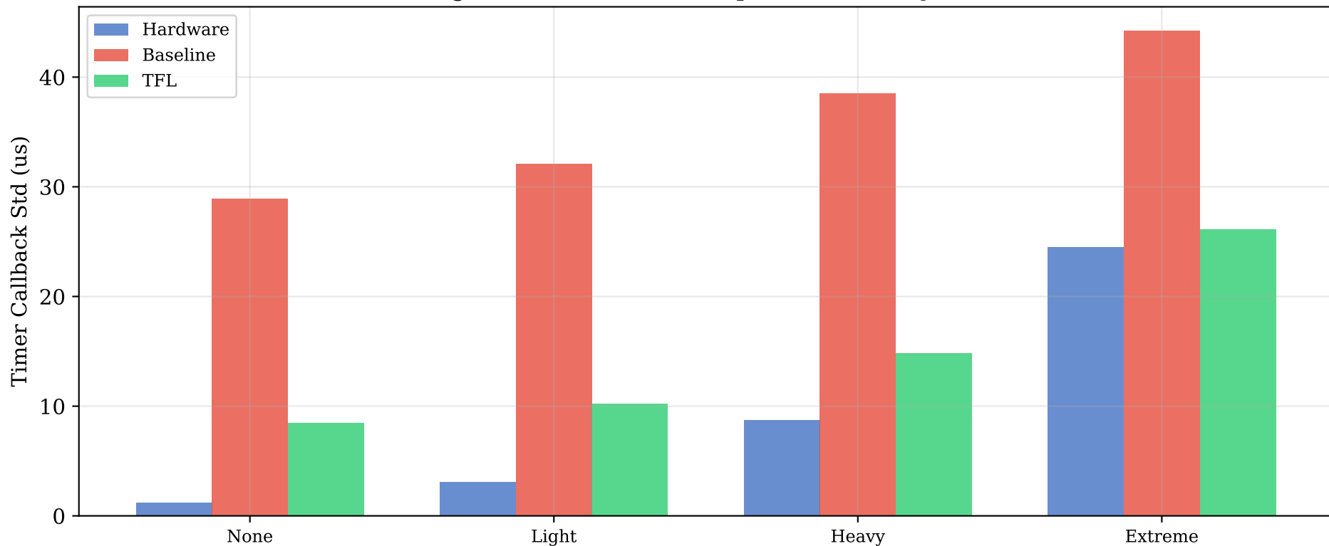
Figure 6.5: Workload Impact on Timer Jitter
