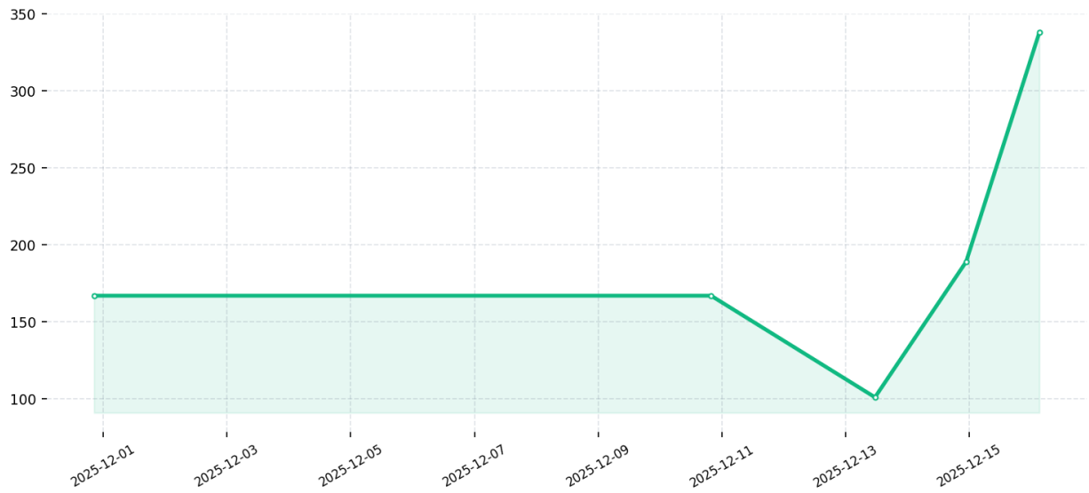
Performance Trajectory
