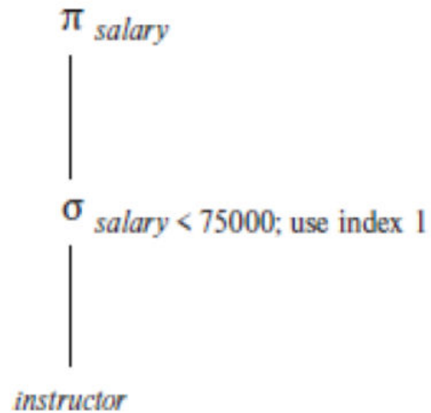
Figure 15.2 A query-evaluation plan.
