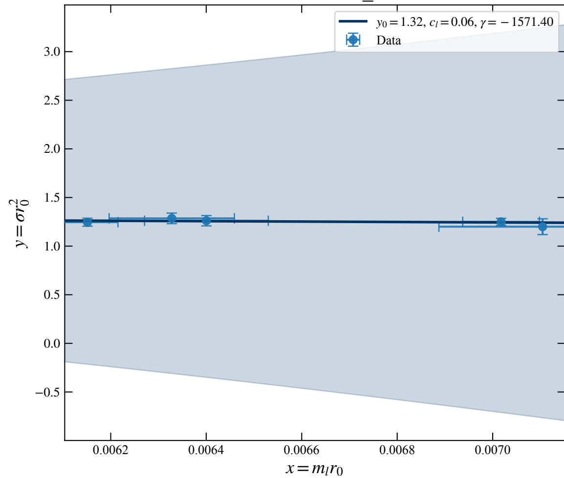
Ensemble: M_i
