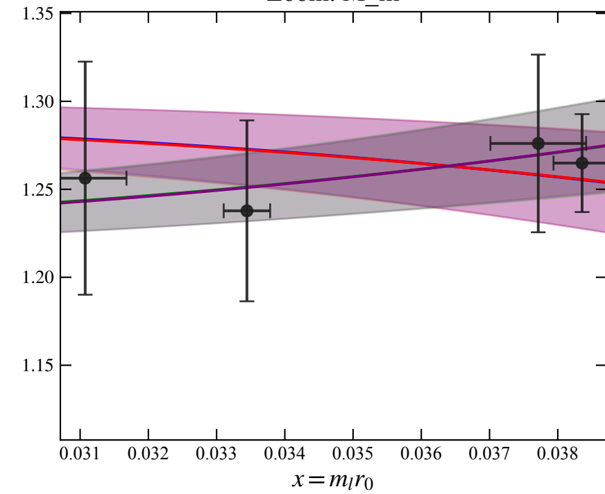
Zoom: M_iii
