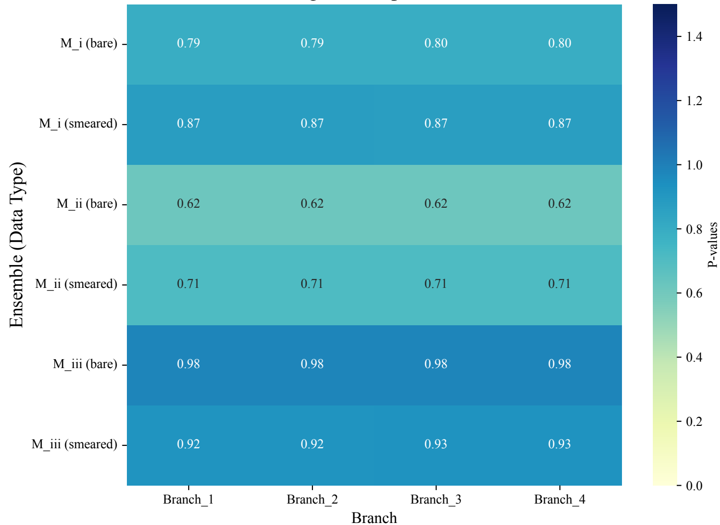
Extended Log Model: p-value ( A = A_{\pi/12} )
