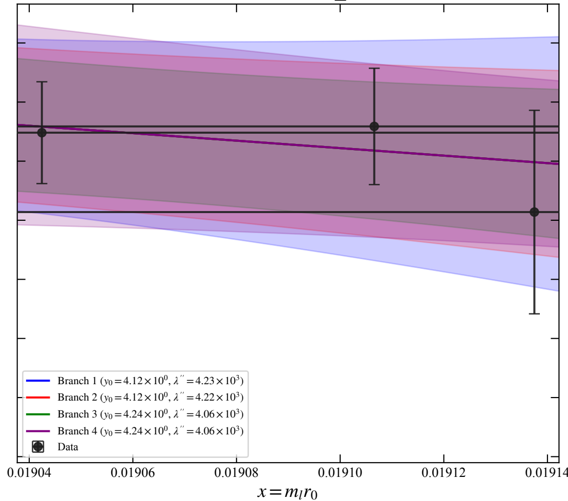
Ensemble: M_ii
