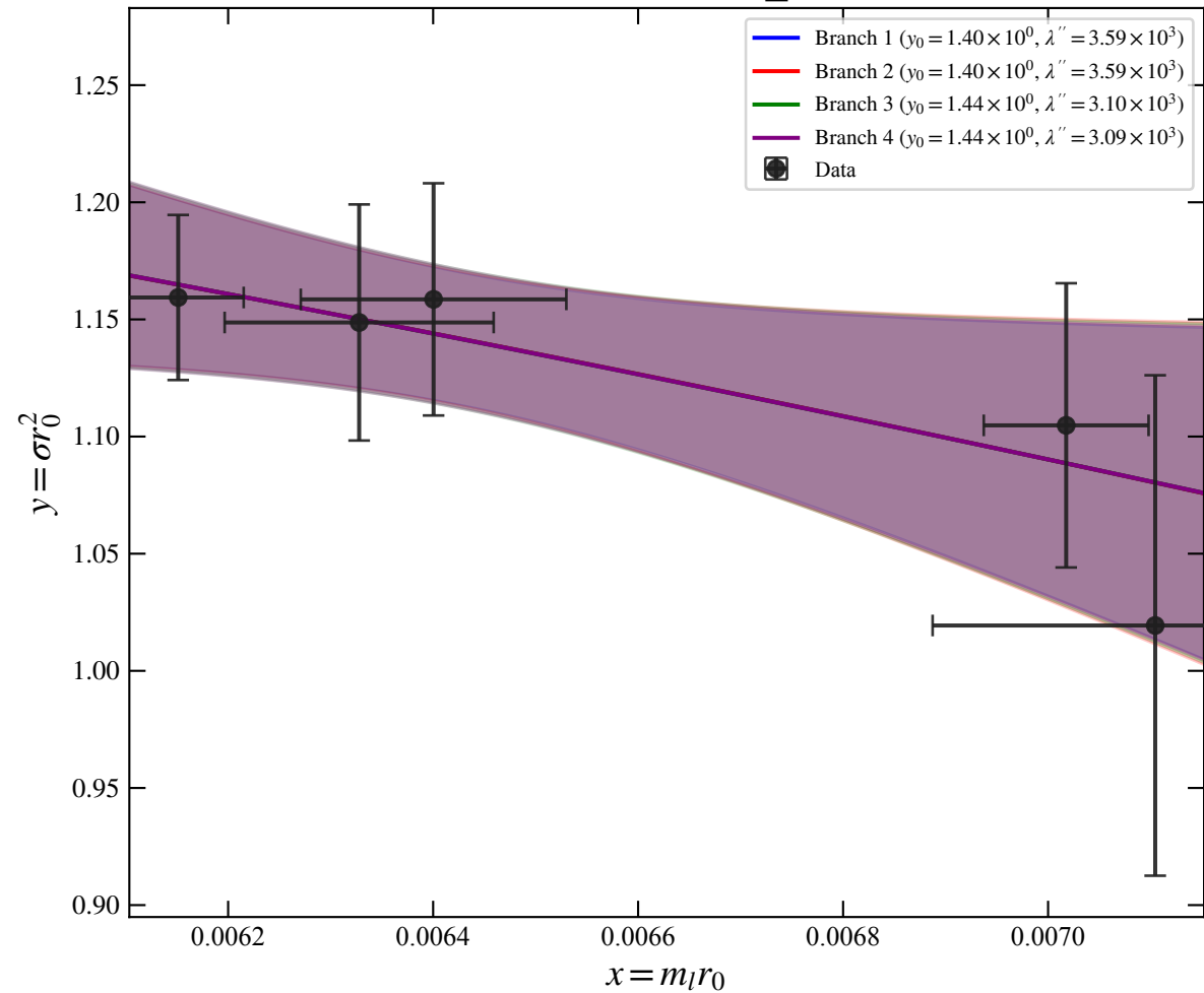
Ensemble: M_i
