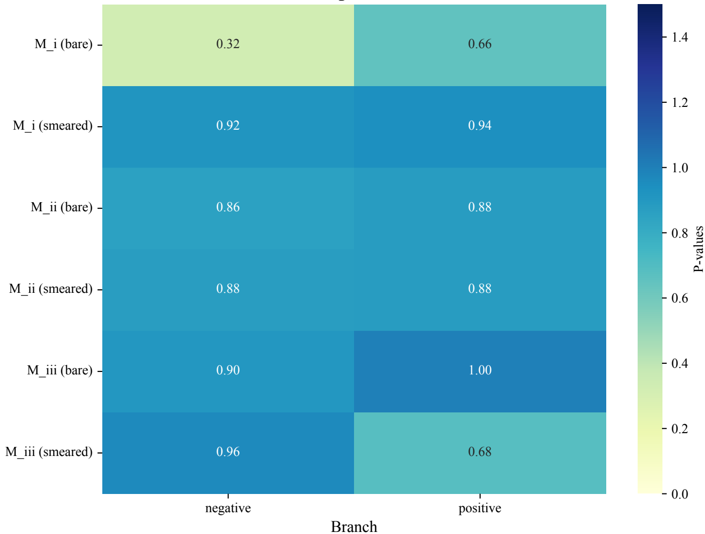
Linear Model: p-value ( A = A_{\pi/12} )
