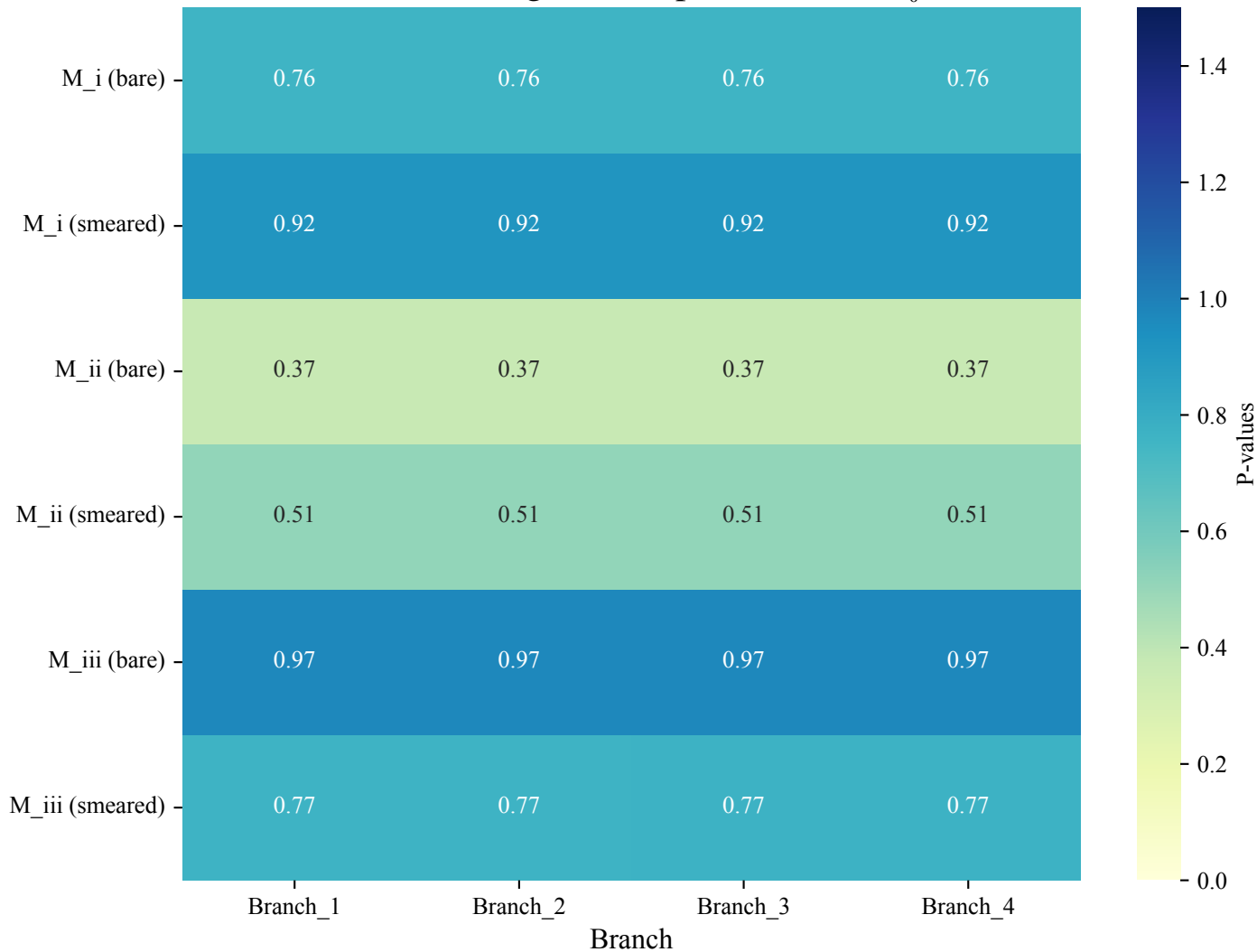
Extended Log Model: p-value ( A = A_{r_0} )
