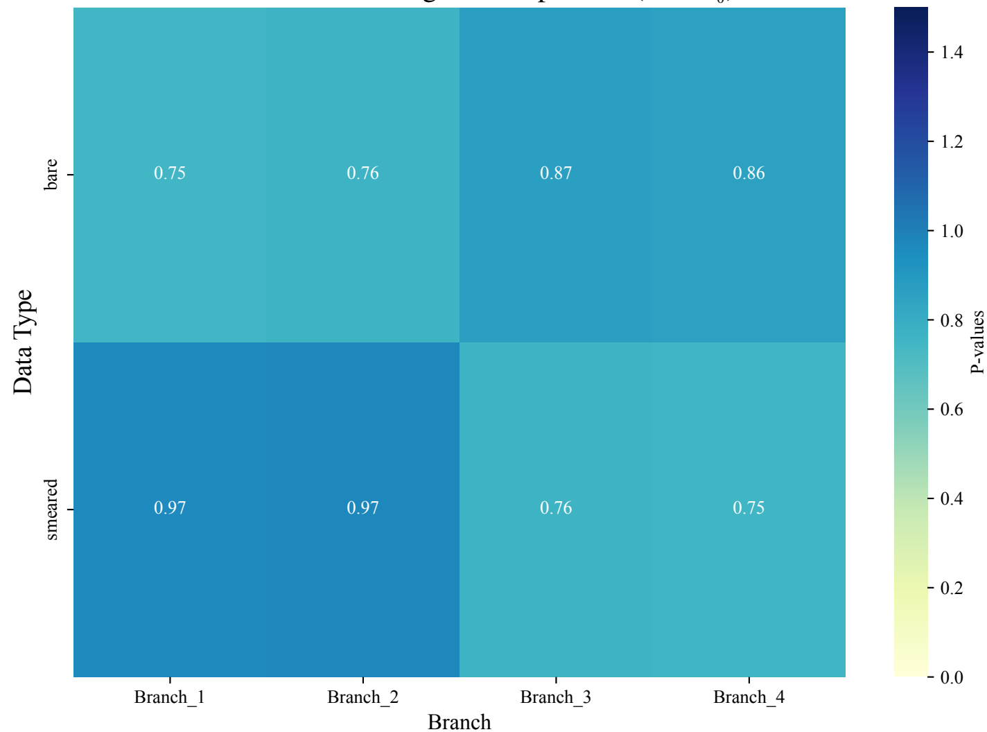
Global Extended Log Model: p-value ( A = A_{r_0} )
