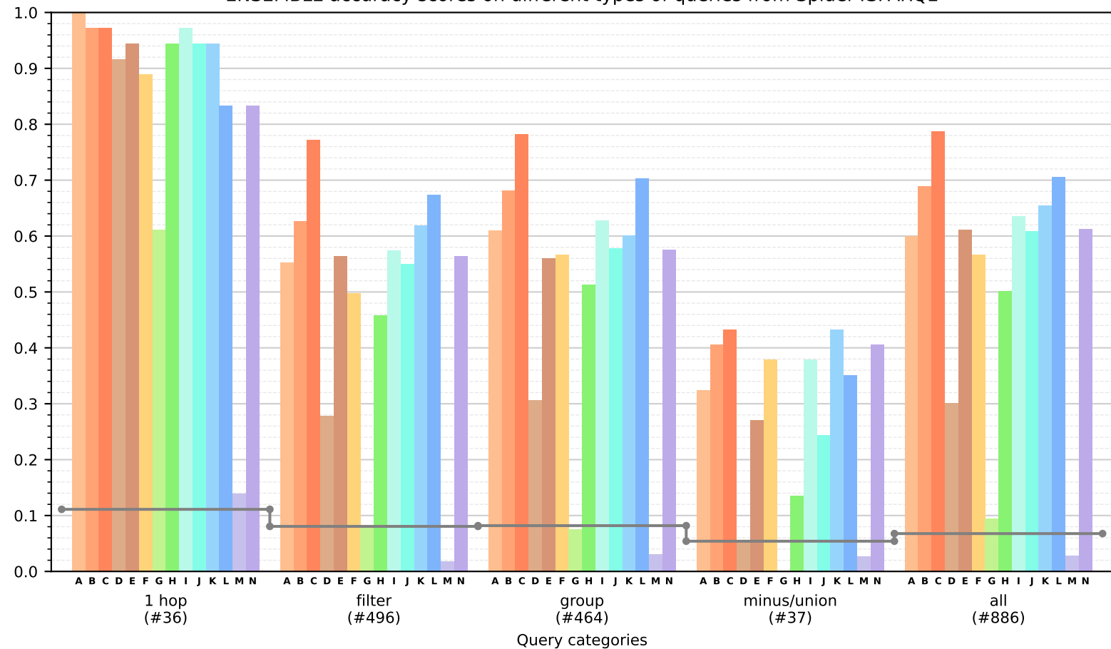
ENSEMBLE accuracy scores on different types of queries from Spider4SPARQL
