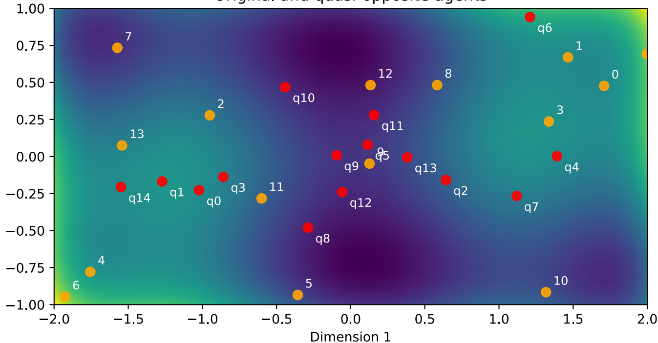
Original and quasi-opposite agents
