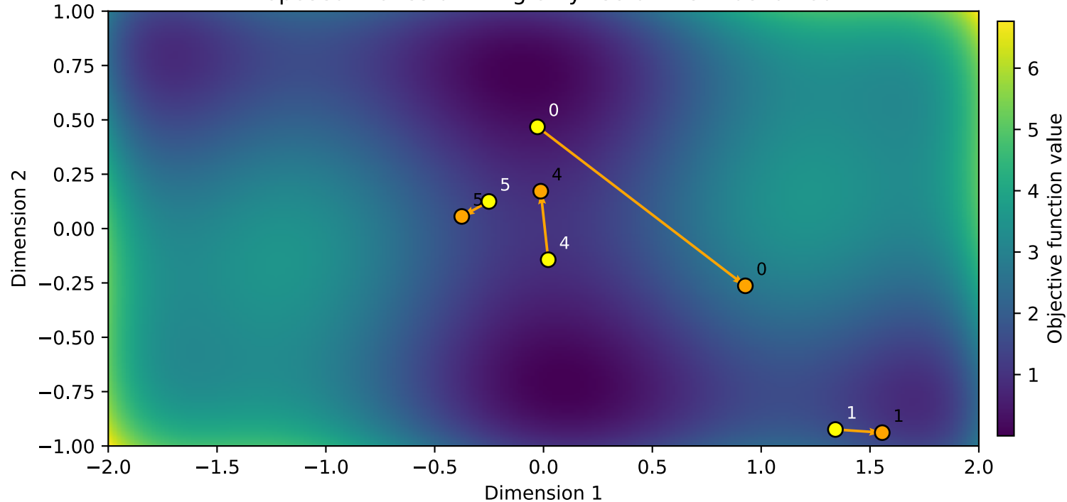
Proposed moves utilizing only recruitment behaviour
